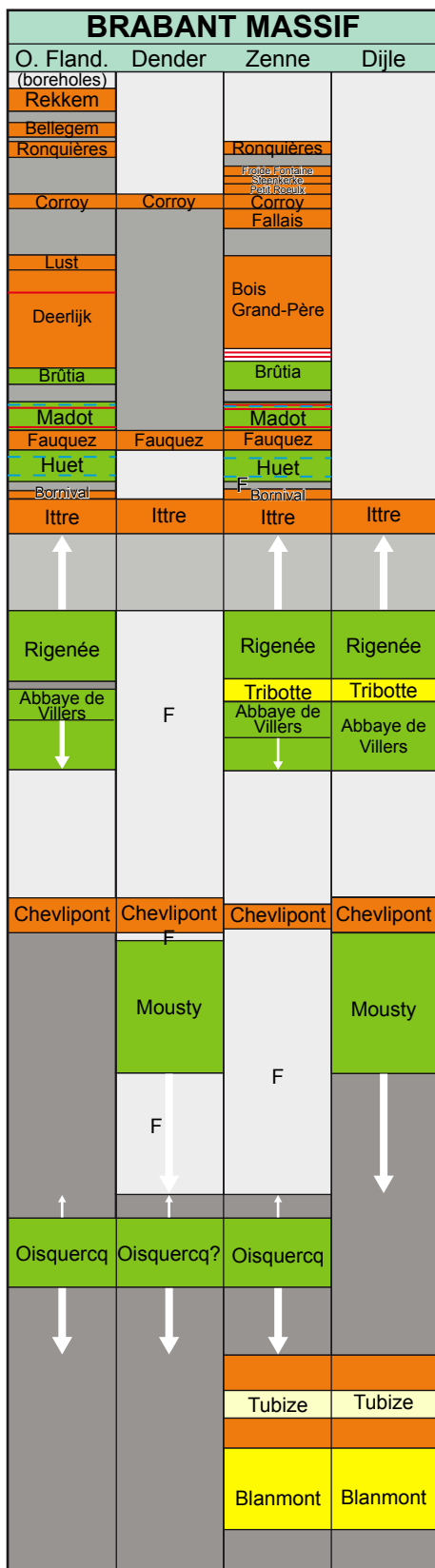
Chronostratigraphic position of the Lower-Paleozoic units in Flanders (after Verniers et al., 2001)
